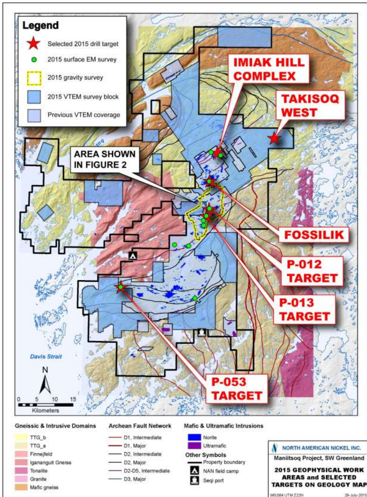
Figure 1: Location of 2015 geophysical work and selected exploration targets.
