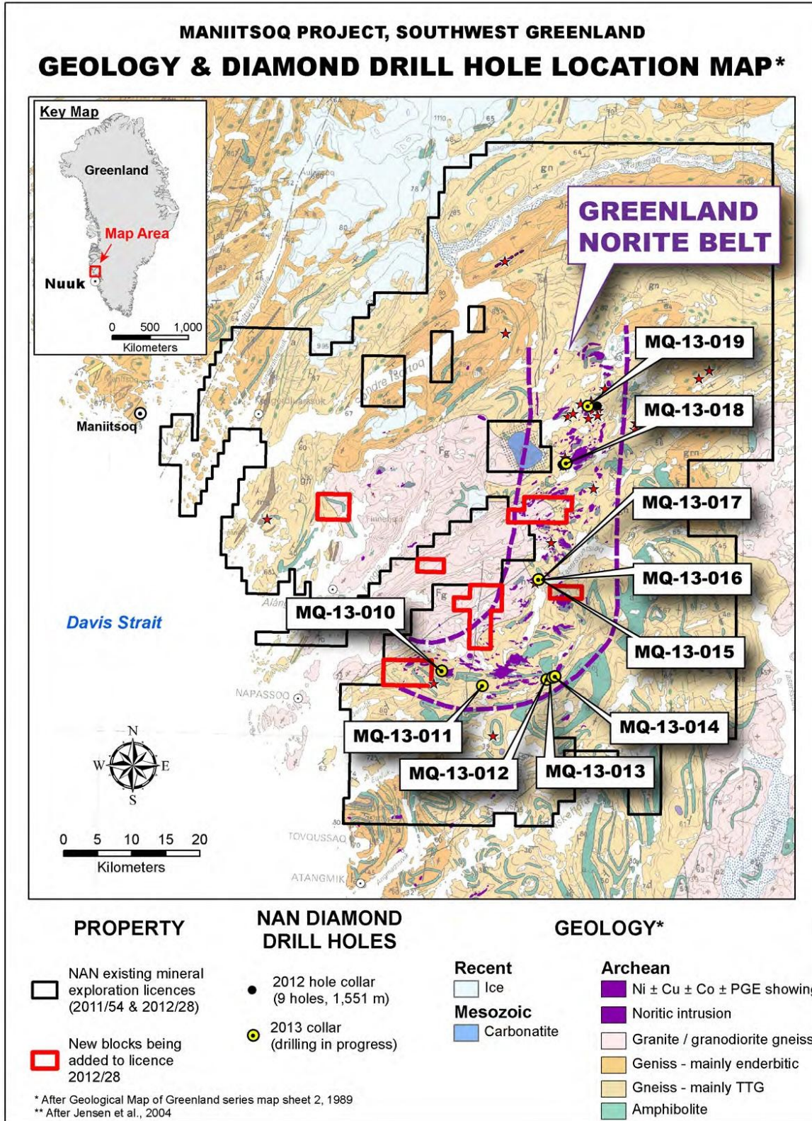
"Figure 1: Geology & Diamond Drill Hole Location Map"
